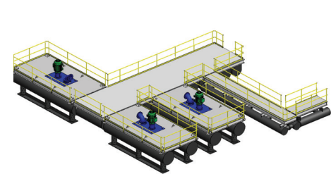
Multiple Pump Open Air Floating Barge
